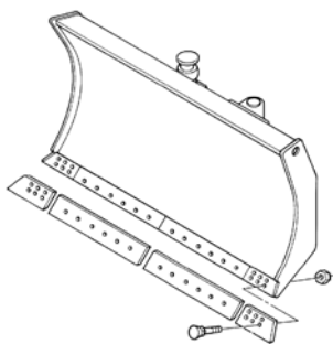
SINGLE BLADE
